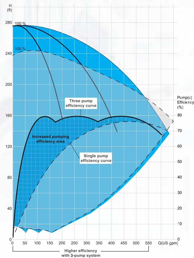
Comparing the three-pump efficiency curve to the single-pump curve reveals a significant increase in efficiency for this multipump system example.
